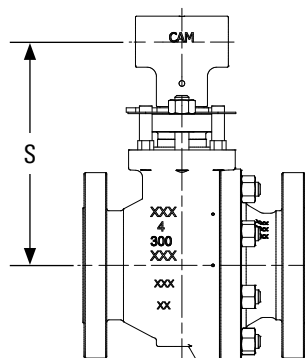
Valve with wrench head.
