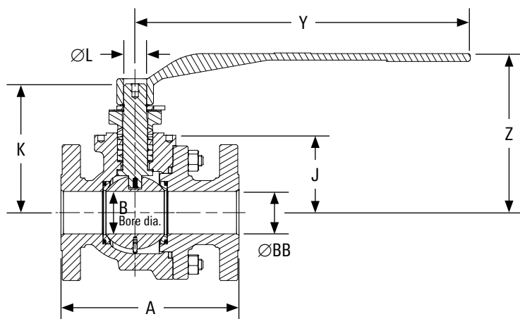
Valve with wrench (lever).
