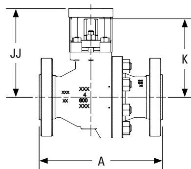
2-in 600 valve with bracket.
