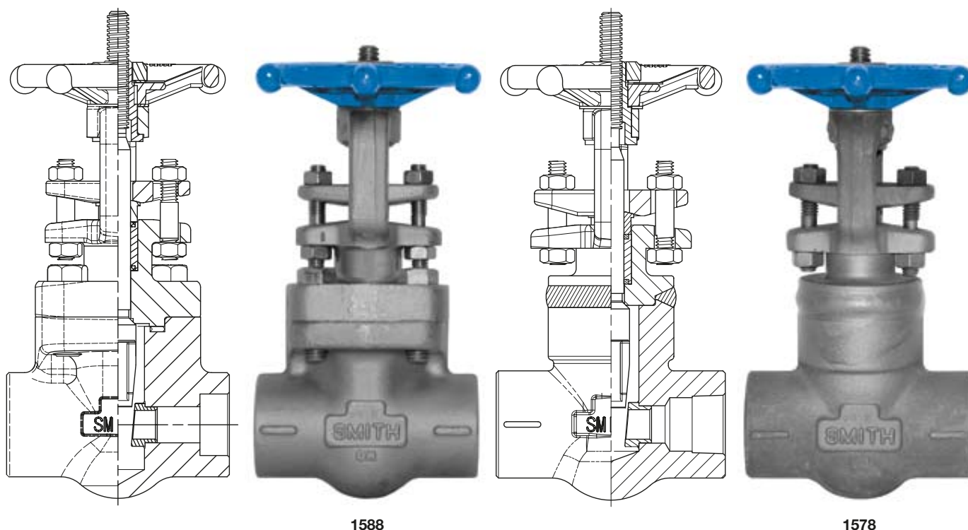
CLASS 1500 FULL PORT BOLTED BONNET GATE VALVE - THREADED or SOCKET WELD - INCHES (MM)
