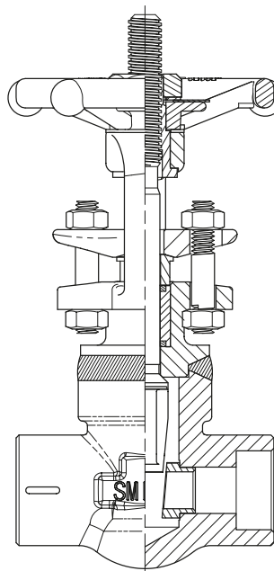
CLASS 800 FULL PORT BOLTED BONNET GATE VALVE - THREADED or SOCKET WELD - INCHES (MM)
